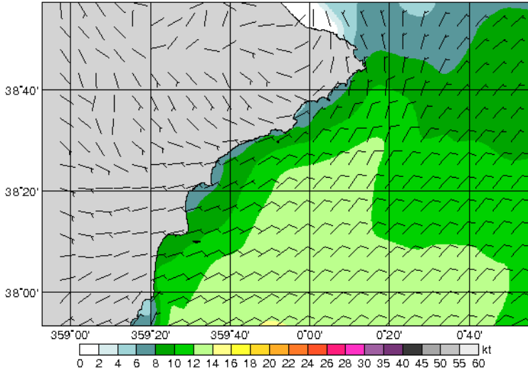
10m Wind speed and direction (kt) 15 Z - 29/08/2008
