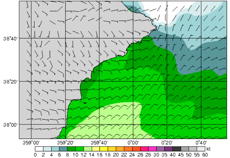
10m Wind speed and direction (kt) 18 Z - 29/08/2008
